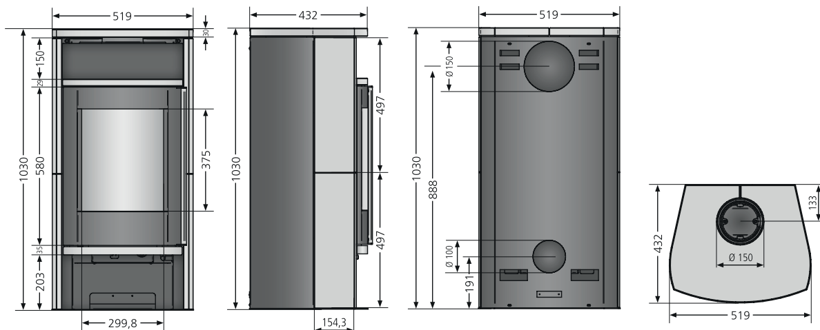
Frisco 2.0, steel black, cover plate and warming compartment in soapstone
